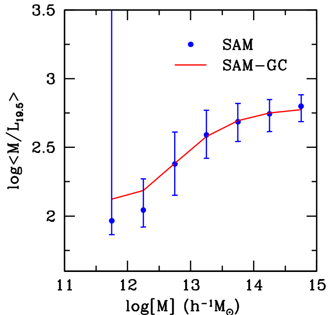
Figure 2. The average mass-to-light ratio, \langle M/L_{19.5} \rangle as a function of halo (group) mass. Here L_{19.5} is the total luminosity of all galaxies in a halo with ^{0.1}M_r - 5 \log h \leq -19.5 . Filled circles with errorbars (indicating the 68 % confidence level) show the results obtained from the SAM directly, using the original halo masses and halo membership. The solid line shows the \langle M/L_{19.5} \rangle as obtained from the SAM group catalogue, and is thus based on the assigned group masses and the assigned group memberships. The agreement with the true \langle M/L_{19.5} \rangle is excellent, indicating that our group finder allows an accurate recovery of the average relation between mass and light.
