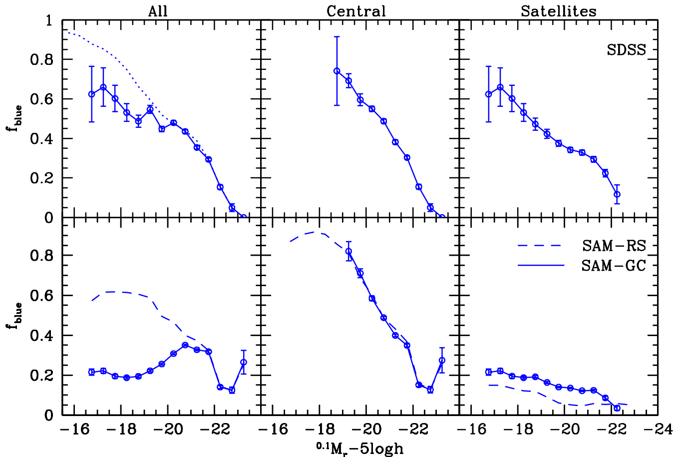
Figure 4. The luminosity dependence of blue galaxy fractions. From left to right, the panels show the blue fractions of all galaxies (centrals plus satellites), central galaxies, and satellite galaxies. The top panels show the results from the SDSS group catalogue (open circles with Poissonian errorbars). The dotted line in the top-left panel shows the results obtained from the full SDSS, including those galaxies that were not assigned to a galaxy group by the group finder. The bottom panels show the results from the SAM of C06. Results are shown for both the SAM-RS (dashed lines) and the SAM-GC (open circles with Poissonian errorbars). See Section 4.2 for a detailed discussion.
