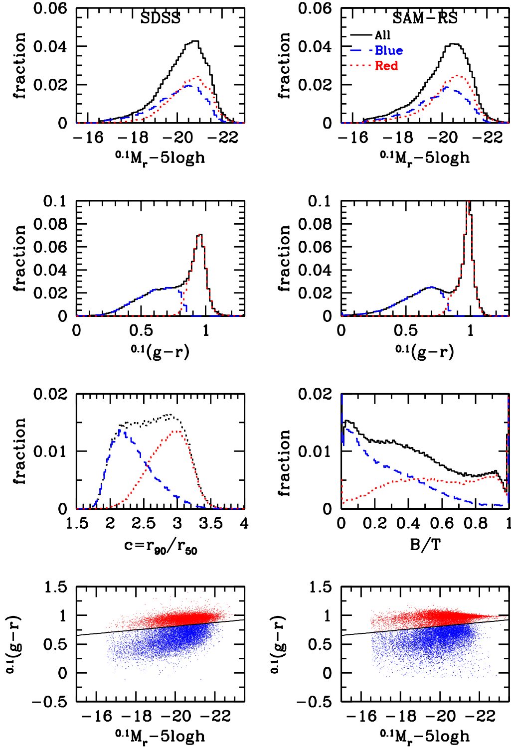
Figure 1. A comparison of global statistics of the SAM-RS (right-hand panels) with the SDSS (left-hand panels). Panels in the first and second row show histograms of absolute ^{0.1}r -band magnitude and ^{0.1}(g-r) colour for both redshift surveys. The contributions from blue and red galaxies are indicated by dashed and dotted lines, respectively. Note the good agreement between SDSS and SAM-RS. Panels in the third row show histograms of morphological parameters. In the case of the SDSS, we plot the distribution of the concentration parameter c , defined as the ratio of the radii containing 90 and 50 percent of the petrosian flux. In the case of the SAM-RS, we plot the distribution of the bulge-to-total mass ratio B/T . Although these can not be compared directly, in general a more concentrated galaxy (higher c ) will also have a larger B/T . Again, the contributions from red and blue galaxies are indicated. Finally, the fourth row of panels shows the colour-magnitude relations. The solid line indicates the bimodality scale given by equation (1), which we use to split the population of galaxies in red and blue subpopulations.
