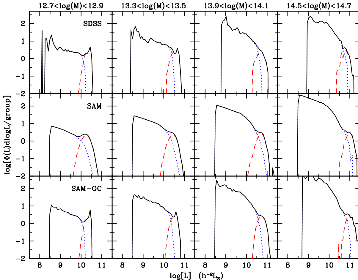
Figure 3. The conditional luminosity function obtained from the SDSS group catalogue (upper panel) from the SAM directly, using true halo masses and true halo members (middle panel) and from the SAM group catalogue, using assigned group masses and assigned memberships (lower panels). Results are shown for four different mass bins (masses in h^{-1} M_{\odot} ), as indicated at the top of each column. Luminosities are in the ^{0.1}r -band. The dotted (blue) line marks the contribution from the satellite galaxies, the dashed (red) line the contribution from the central galaxies.
